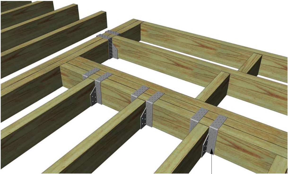
ceiling joist supporting detail
