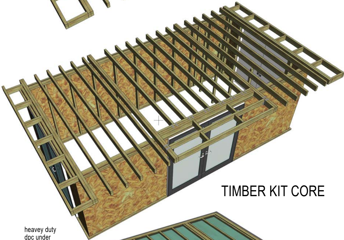
ROOF JOISTS LAYOUT
